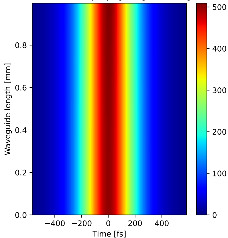
Evolution of Pulse propagating in Waveguide
